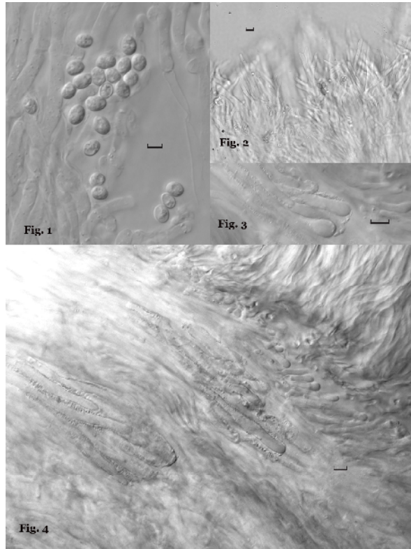
Figures 1-4. Aurantiopileus mayanensis . T. J. Baroni 10228 : Fig. 1. Basidiospores at 1000x, DIC. Scale bar = 5 \mu\text{m} . Fig. 2. Sterile cells on pore edges at 400x, DIC. Scale bar = 10 \mu\text{m} . Fig. 3. Embedded tramal cystidia at 1000x, DIC. Scale bar = 20 \mu\text{m} . Fig. 4. Embedded tramal cystidia at 400x, DIC. Scale bar = 10 \mu\text{m} .
