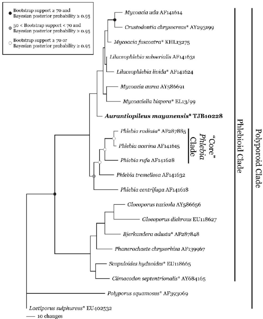
Figure 6. Inferred phylogeny based on nLSU. The tree shown is one of 58 equally parsimonious trees (Length = 461, CI = 0.60, RI = 0.49). Statistical support for nodes is based on parsimony and Bayesian analyses. The asterisk after a name indicates that it is the type species of that genus.
